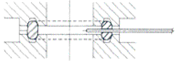
Ring-Type Joint
