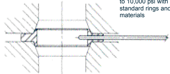
Seal Ring
